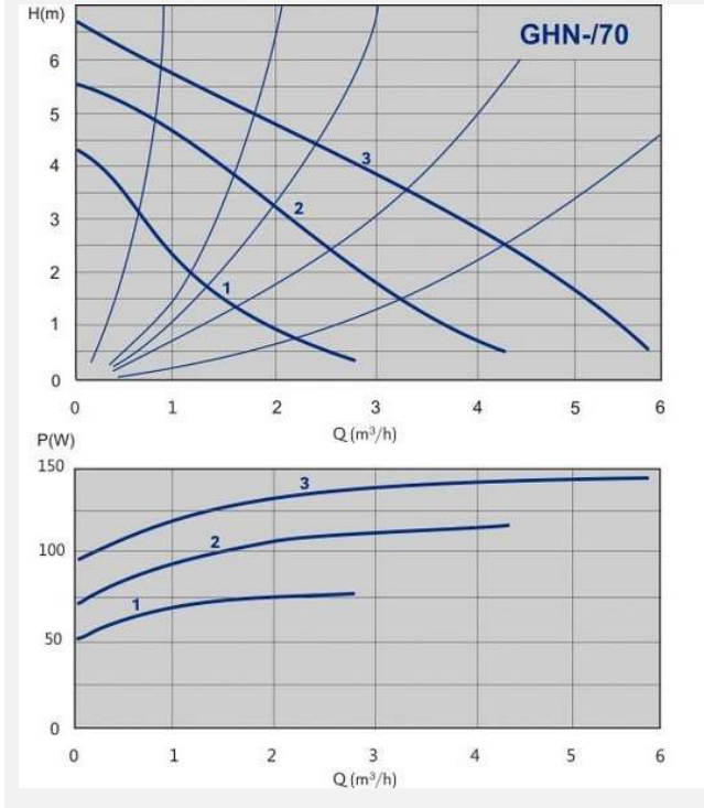
Pumpe mobiheat GHN 25/70
